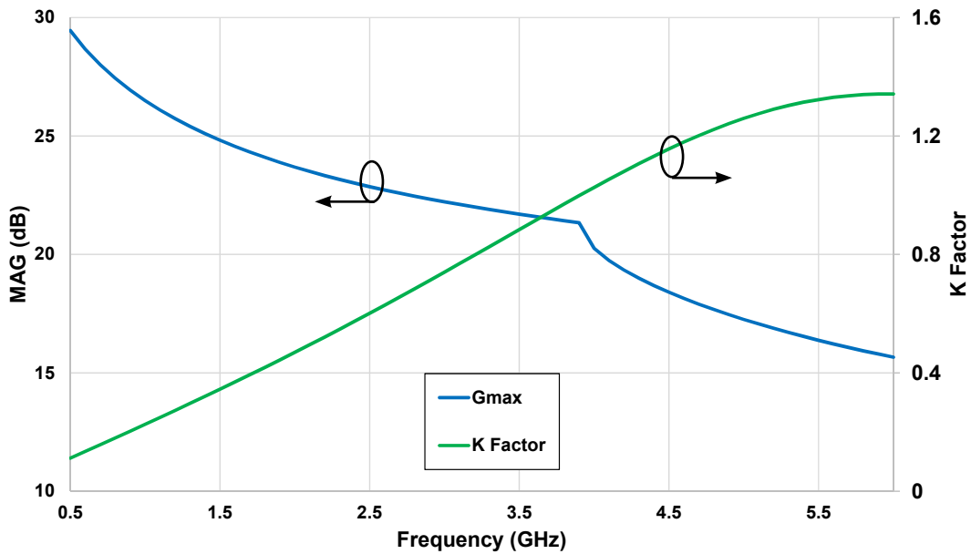
Maximum Available Gain and K Factor of the CG2H40025
